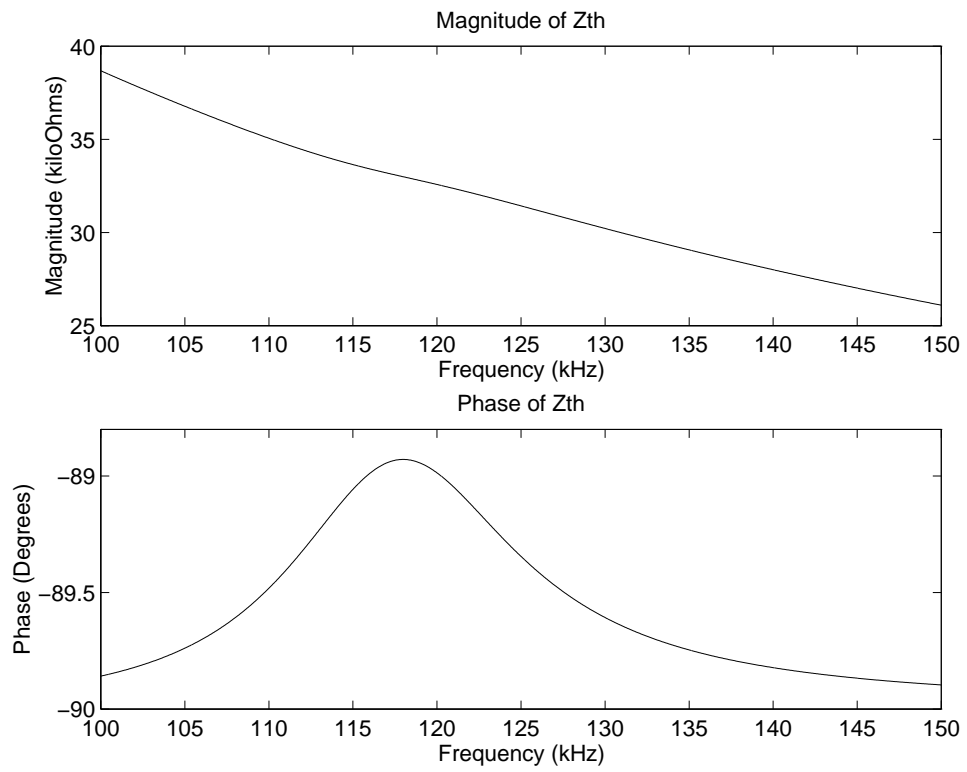
Figure 3-3: Magnitude and Phase of Z_{th} as a function of f_r with R = 50 \text{ k}\Omega .
