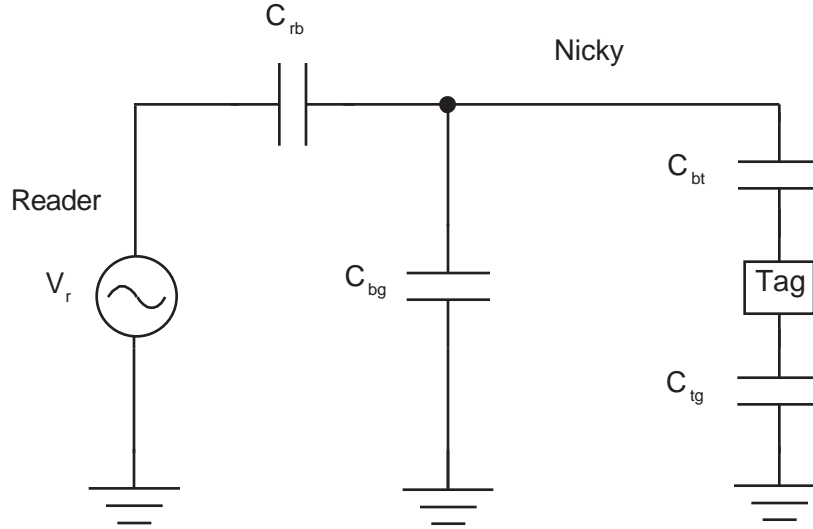
Figure 2-1: The electrostatic model of the reader, body, and tag interaction.
