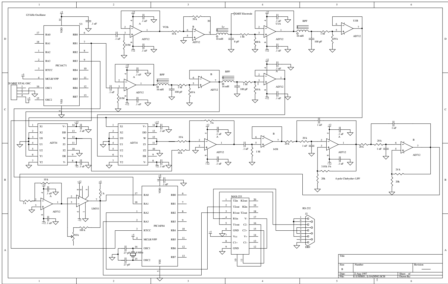
Figure B-1: Loading mode reader schematic.
