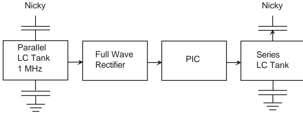
Figure 4-1: Block diagram of the transmit mode bodytag.
