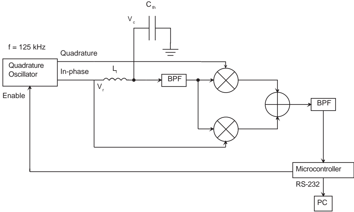
Figure 3-5: Block diagram of the loading mode reader.
